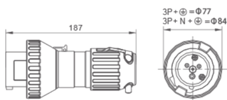
Plugue
