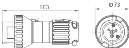
Plugue
